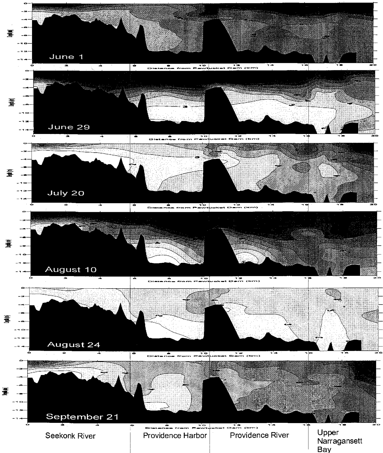
Figure 13: Tidally averaged dissolved oxygen vs. depth and location during the 1995 surveys. White areas: <math>< 2 \text{ mg/l}</math>. Green areas: <math>2\text{--}3 \text{ mg/l}</math>. Blue areas >math>3 \text{ mg/l}</math> at 1mg/l increments.
